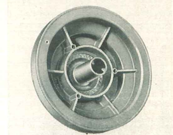
The pulley is carried on a large sealed-for-life ball bearing, requiring no lubrication, and with a load capacity far in excess of any pulley ever placed on it by the belt.
